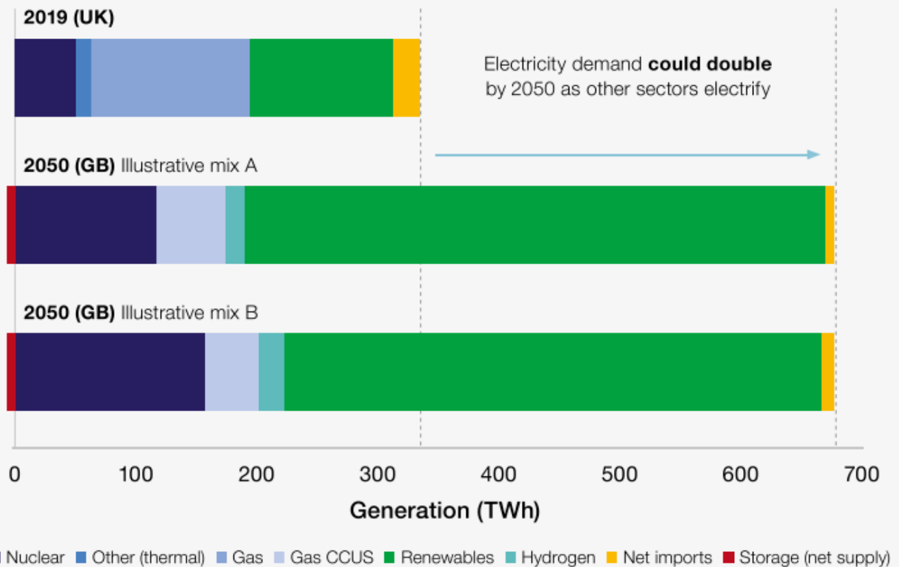
FIGURE 3.4 - ELECTRICITY MIX TODAY & ILLUSTRATIVE 2050 MIXES
